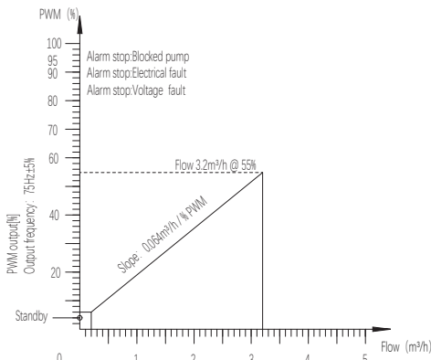
Fig. 9 Feedback PWM signal
