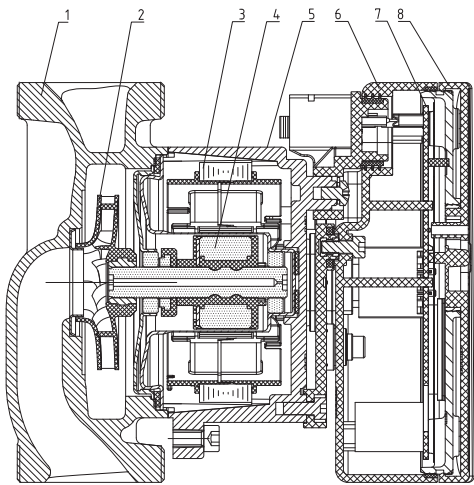
Fig. 13 Sectional drawing
