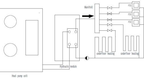
Fig.5 Heat pump system
