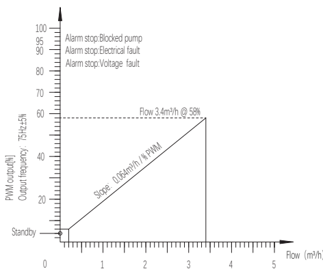
Fig. 10 Feedback PWM signal
