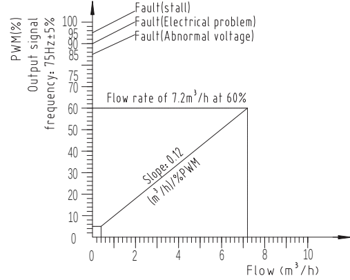
Fig. 10 Feedback PWM signal
